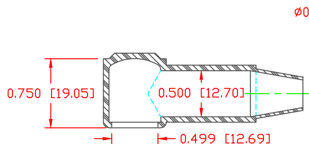
SECTION A-A TYP. WALL THICKNESS = .060" [1.5] SEAL NO. 2 SHOWN
