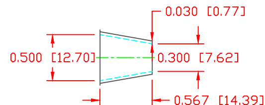
SEAL THICKNESS = .030" [0.8] NO. 2 Cable Gages 8 - 2
