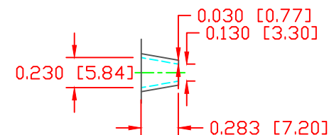
SEAL THICKNESS = .030" [.8] NO. 1 Wire Gages 18 - 10
