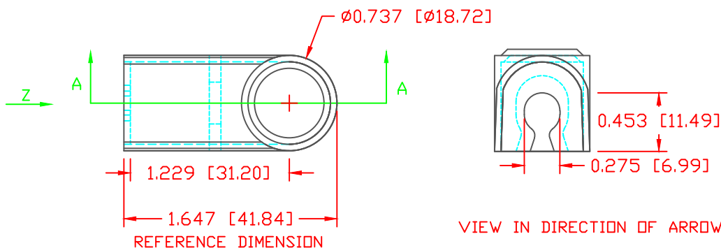
REFERENCE DIMENSION
