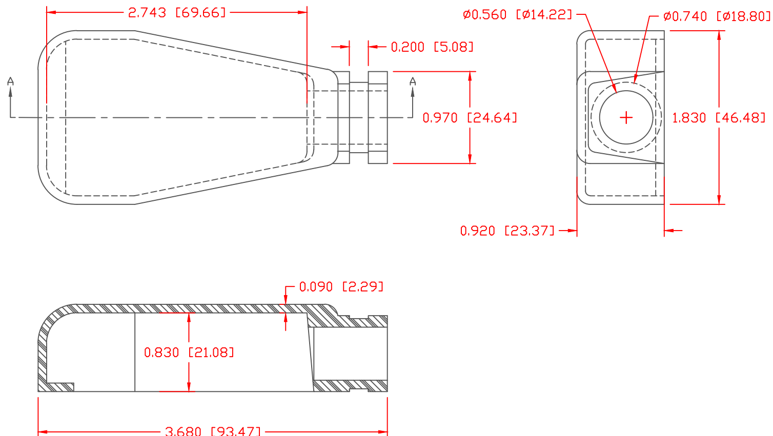
SECTION A-A TYP. WALL THICKNESS = .090" [2.3]
